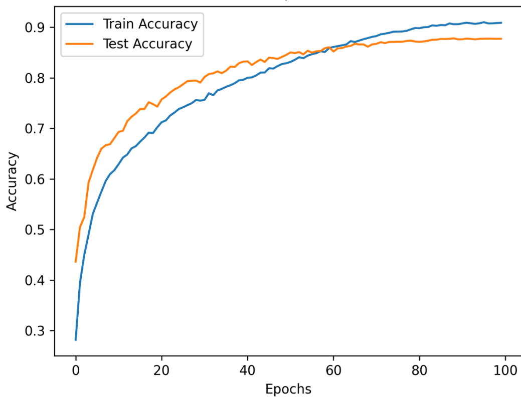
Train and Test Accuracies, Conv Vision Transformer
